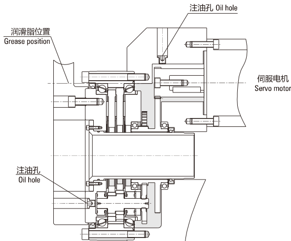
Figure D.6: Lubricating oil injection position (horizontal) (安装水平轴 Install horizontal axis)
